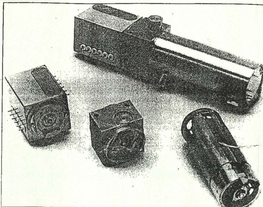
Figure 9. MC2935 Trajectory Stronglink Switch
